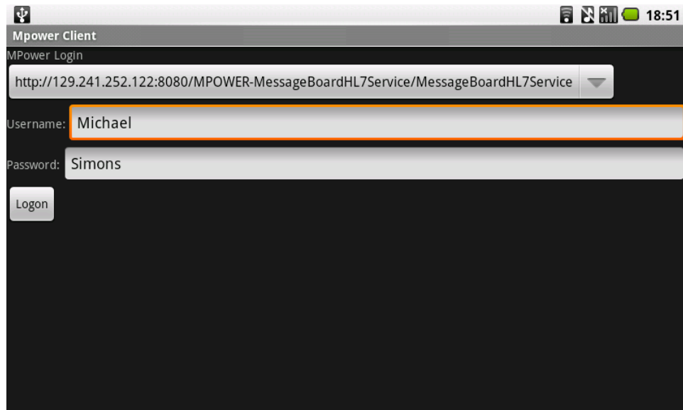
Figure C.1: Authentication screen.
